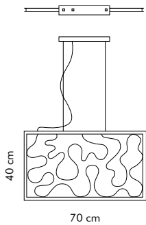
SP 8/282 SP 8/282 V con vetro bianco/with white glass STRIP LED 48W CE
