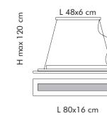
SP M/267 1 x max 55W 2 G11 \rightarrow + STRIP LED 14W \approx + CE IP20 ES
