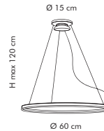
SP 8/267 1 x max 80W ECO R7s \rightarrow 78 mm + STRIP LED 14W \approx + or 1 x max 75W QR111 \rightarrow + STRIP LED 14W \approx + CE IP20 ES
