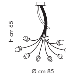
SP 8/225 9 x max 33 W ECO G9
