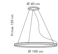
SP S/267 3 x max 75W QR111 \rightarrow + STRIP LED 24W \approx + CE IP20 ES
