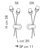
LP 6/225 A sx-dx 2 x max 33 W ECO G9
