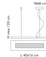
SP H/267 1 x max 80W ECO R7s \rightarrow 78 mm + STRIP LED 7W \approx + CE IP20 ES
