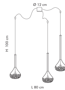
SP 8/276 A 3 x max 25W ECO GY 6,35 \Rightarrow \Leftarrow CE IP20 \square \nabla
