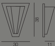
1059/1AP-LN... L 30 x H 38 x Sp. 11 cm E14 1x60W
