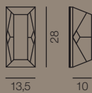
1028/1AP-B... L 13,5 x H 28 x Sp. 10 cm ● E14 1x60W
