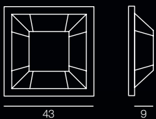
2015/4PL-LN... L 43x43 x Sp. 9 cm E14 4x40W
