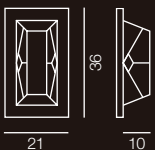
1028/1AP-LN... L 21 x H 36 x Sp. 10 cm ⊙ E14 1x60W
