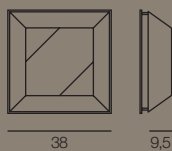
975/4PL-B... L 38x38 x Sp. 9,5 cm ⦿ E14 4x40W
