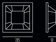
2014/2PL-LN... L 35x35 x Sp. 9 cm E14 2x40W
