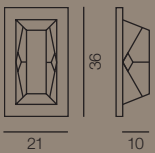
1028/1AP-LN... L 21 x H 36 x Sp. 10 cm ● E14 1x60W
