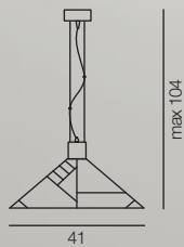
3054/1S... L 41x41 x H max 104 cm E27 1x75W ES
