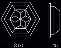
970/5PL-LN... Ø 50 x Sp. 15 cm ◐ E14 5x40W
