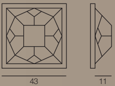
1029/4PL-LN... L 43x43 x Sp. 11 cm E14 4x40W
